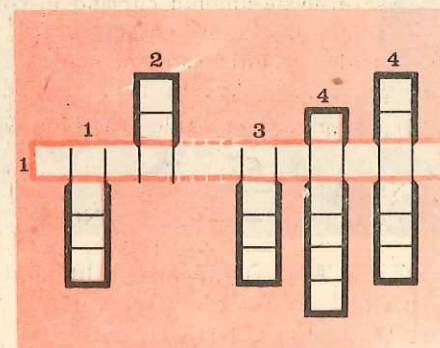
Fig. 4.37. Rebus chimic
