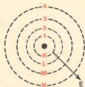
Fig. 1.3. Straturi electronice
