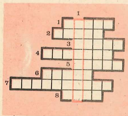
Fig. 7.13. Rebus chimic
