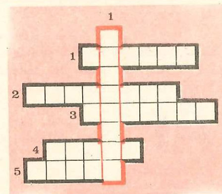
Fig. 8.15. Rebus chimic
